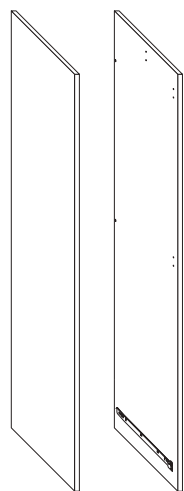
1xA1 + 1xA2 Fianchi sinistro+destra Left+right side panels
